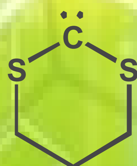
Seebach's Carbene Schreiner, Mloston 2006
